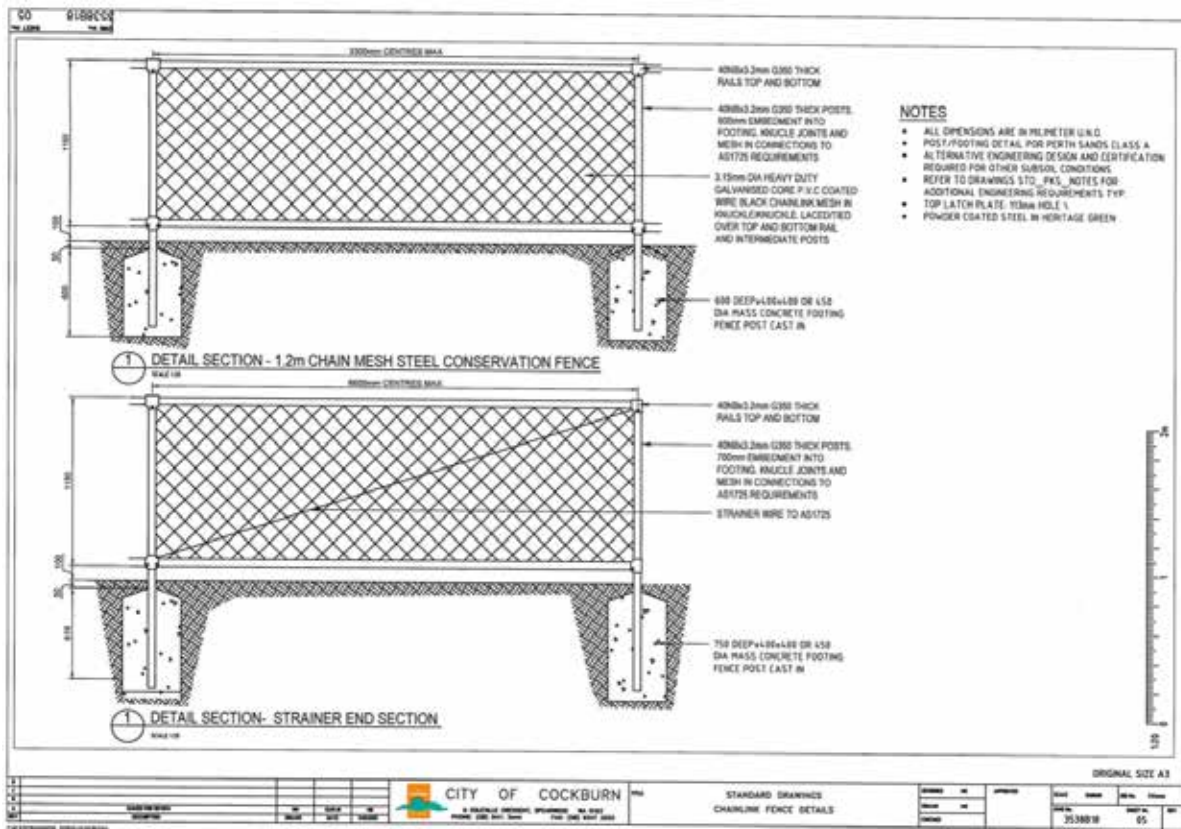
Diagram 1: Type 1 Conservation fence specifications
