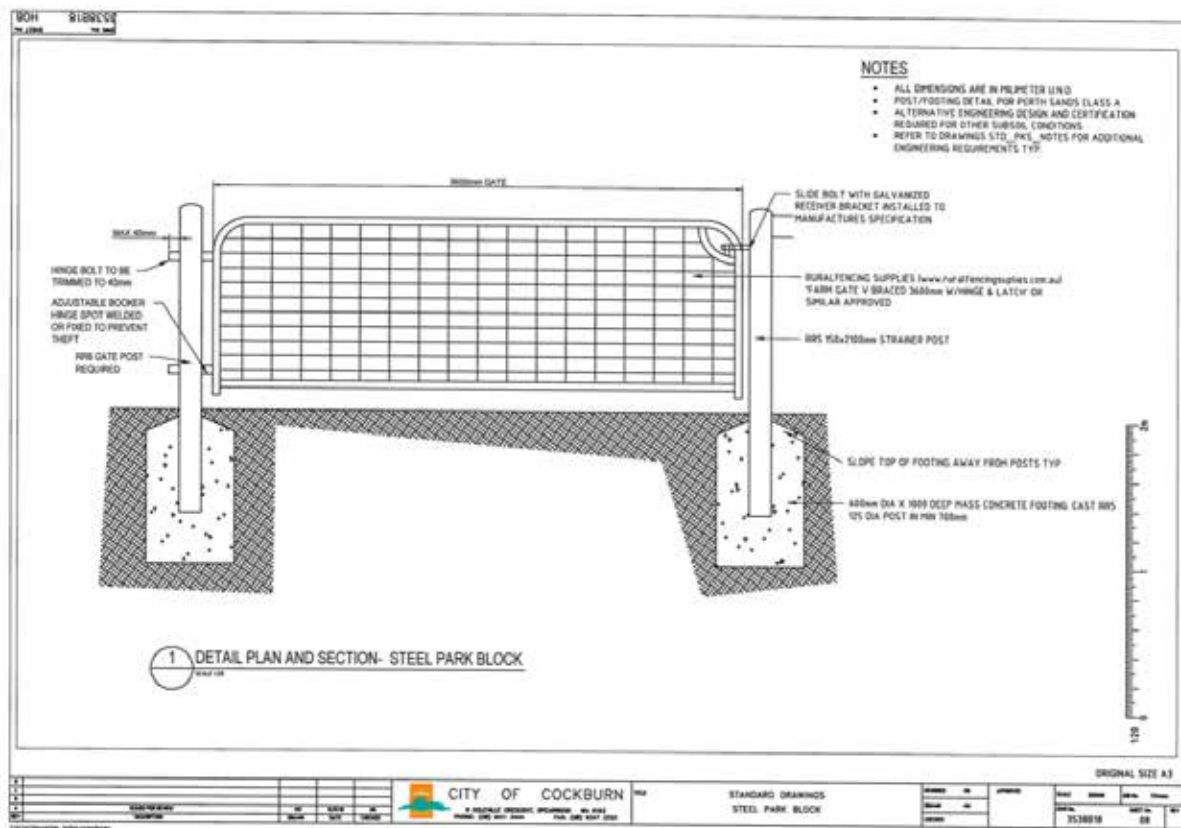
Diagram 3: Conservation gate specification
